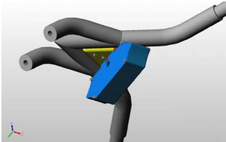
Using the two 10-32 X 3/8" screws, bolt cap to bottom of bars to hold mounting bracket in place.
