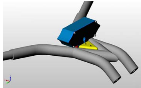
Using the two 10-32 X 3/8" screws, bolt cap to top of bars to hold mounting bracket in place.
