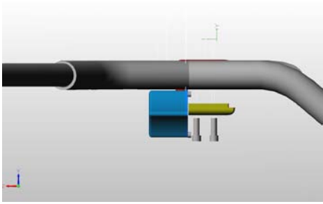
Position bracket and gauge onto bars.
