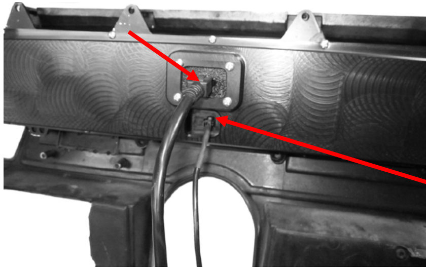
Buzzer Connector
