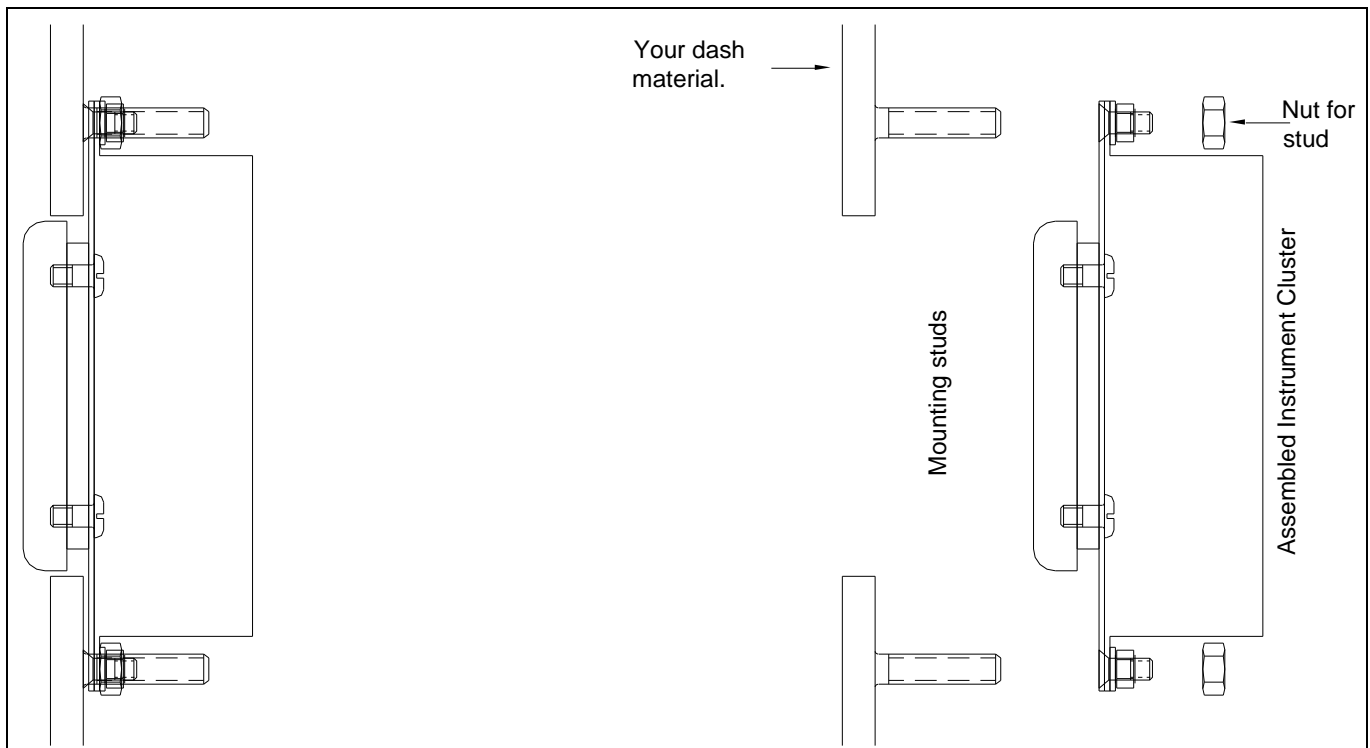
Figure 3. Mounting Method #2.
