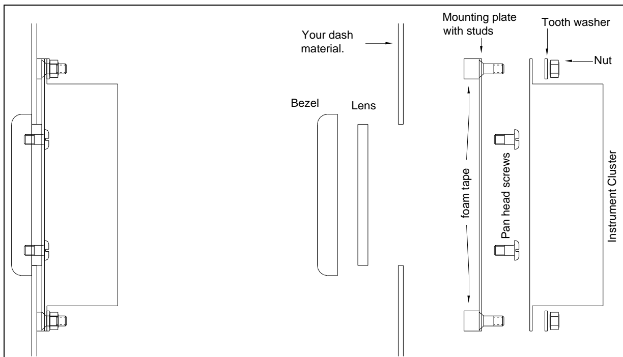
Figure 1. Mounting Method #1 with thin dash.
