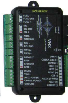
Control Box
