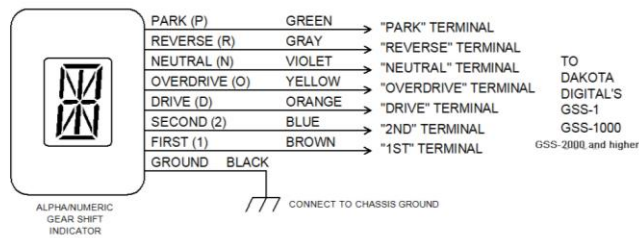
CONNECTION TO DAKOTA DIGITAL'S UNIVERSAL GEAR SHIFT SENDER (GSS-1, GSS-1000 or GSS-2000).
