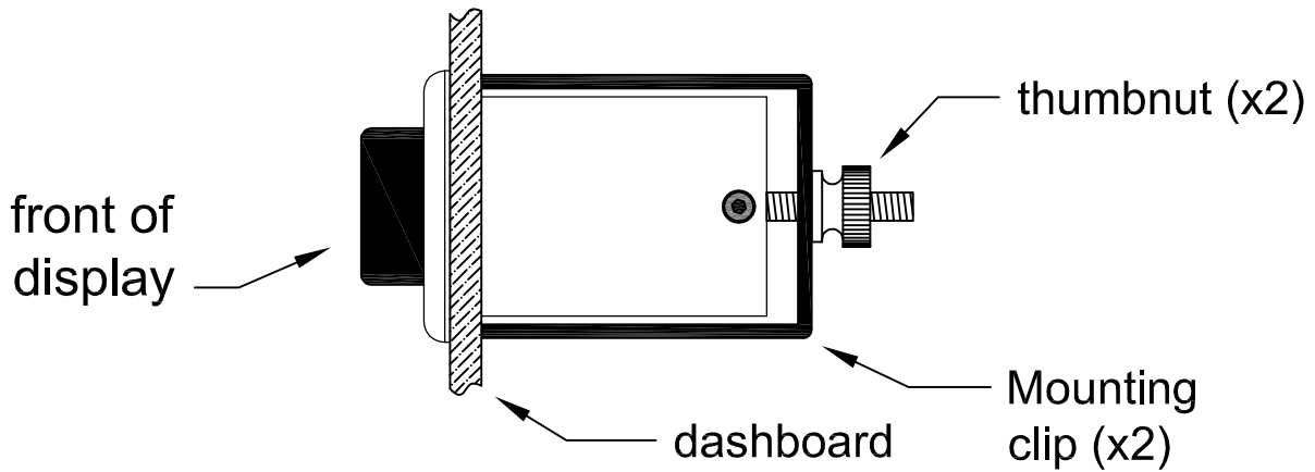
Mounting diagram for DCC-2400/2500/3000 display
