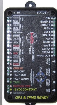
Control Box
