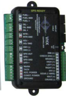
Control Box
