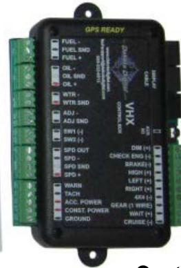
Control Box
